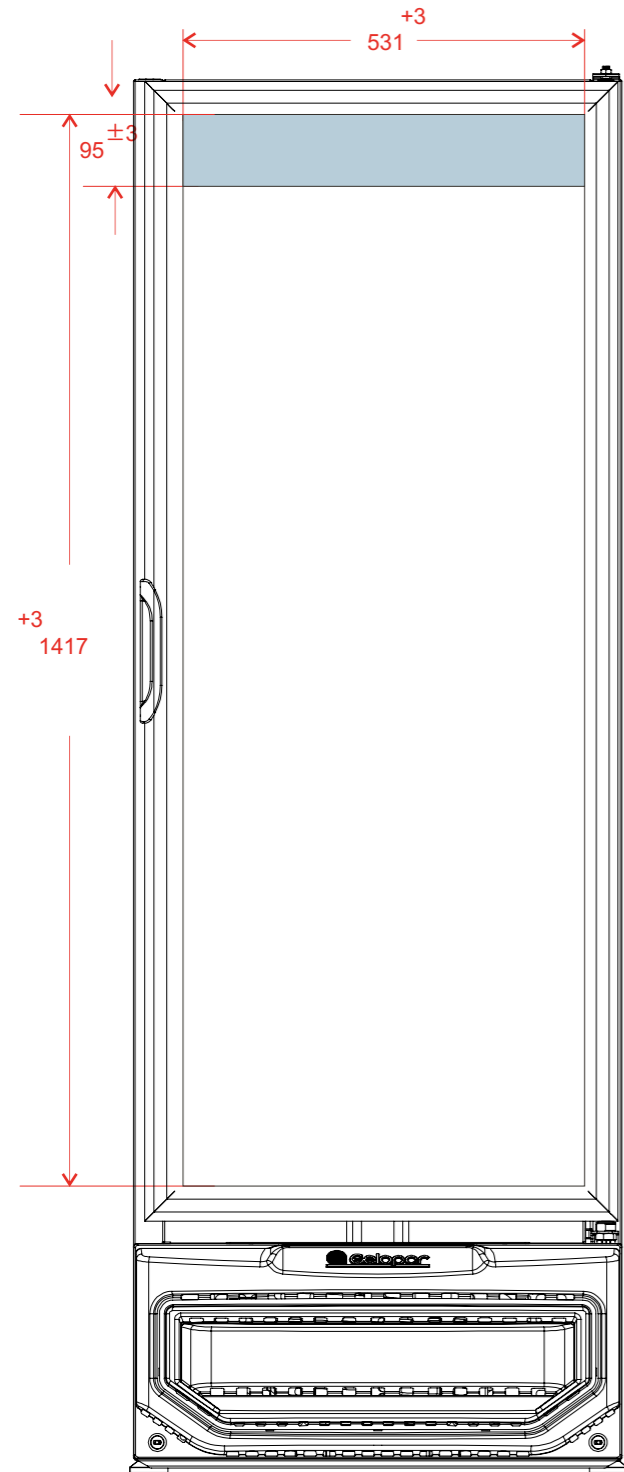
VISTA FRONTAL
